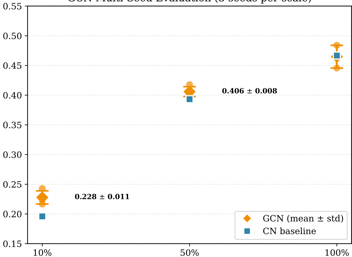
GCN Multi-Seed Evaluation (3 seeds per scale)
